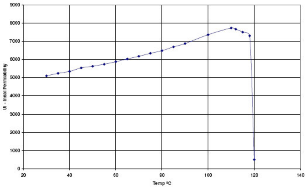
CF195A \mu_i vs Temp
