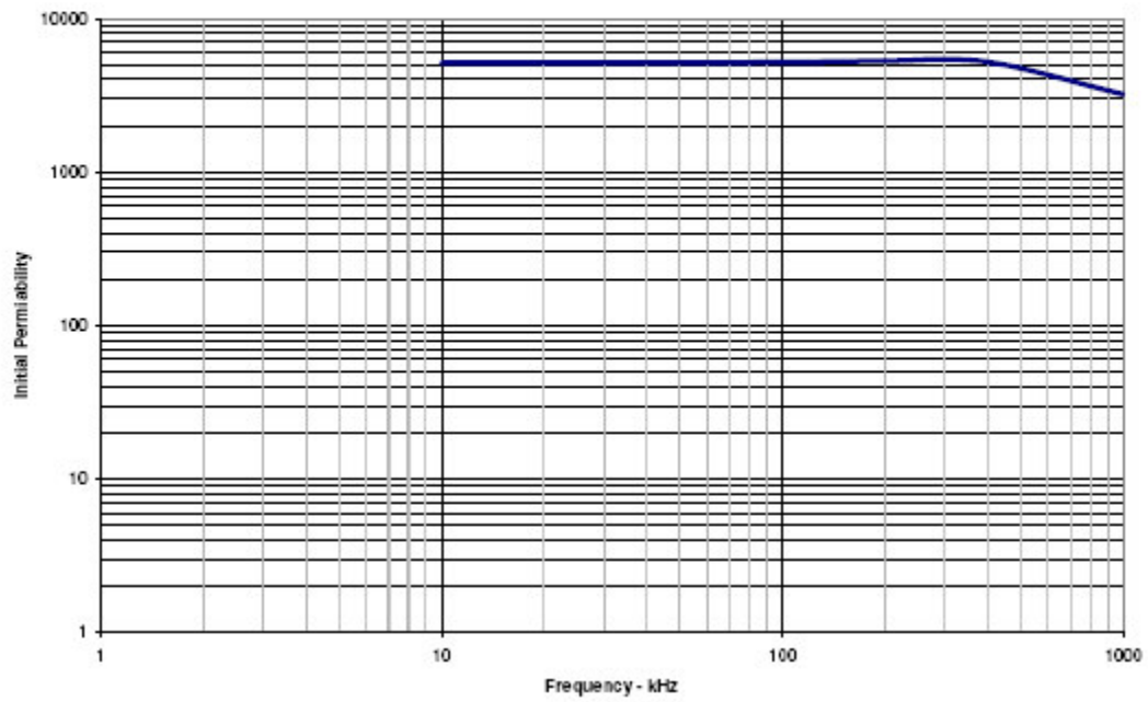
CF195A Initial Permiability vs Frequency
