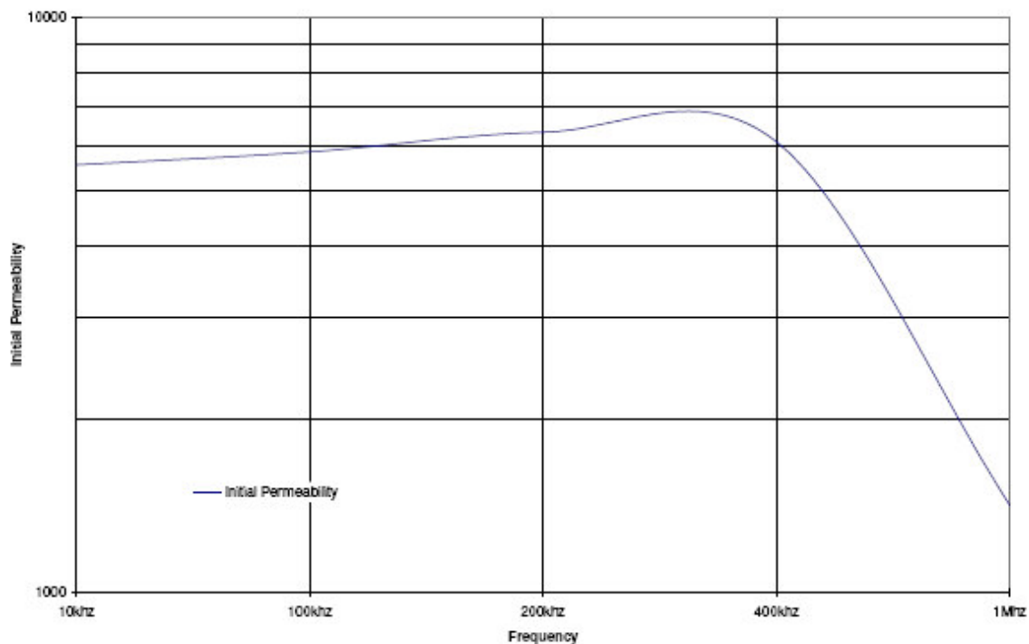
CF255 Initial Permeability Vs Frequency
