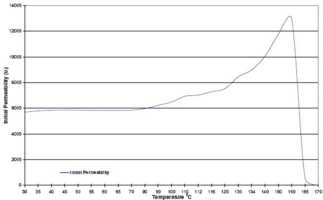
CF255 Curie Plot
