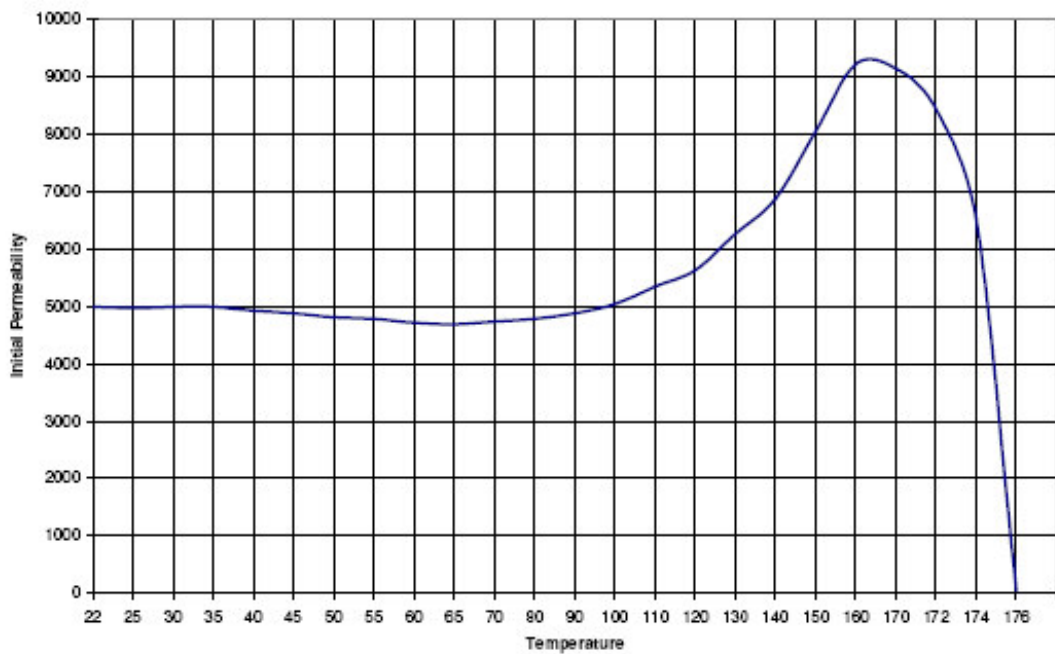
CF265 Initial Permeability Vs Temperature
