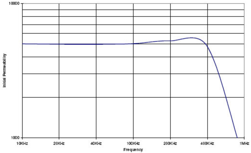
CF265 - Initial Permeability Vs Frequency
