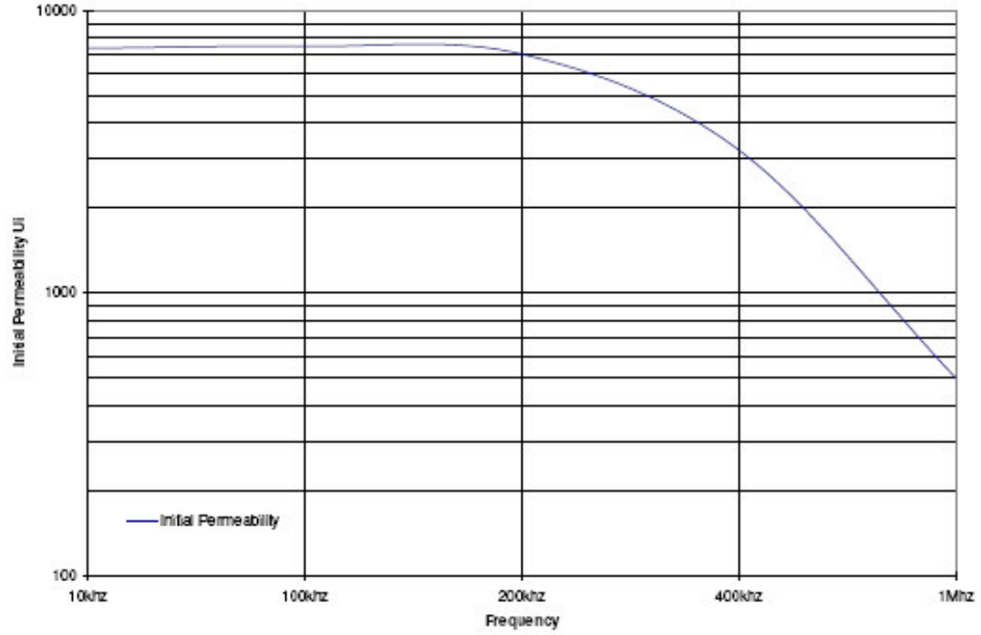
Initial Permeability Vx Frequency
