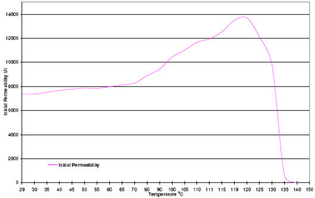
CF275 Curie Plot
