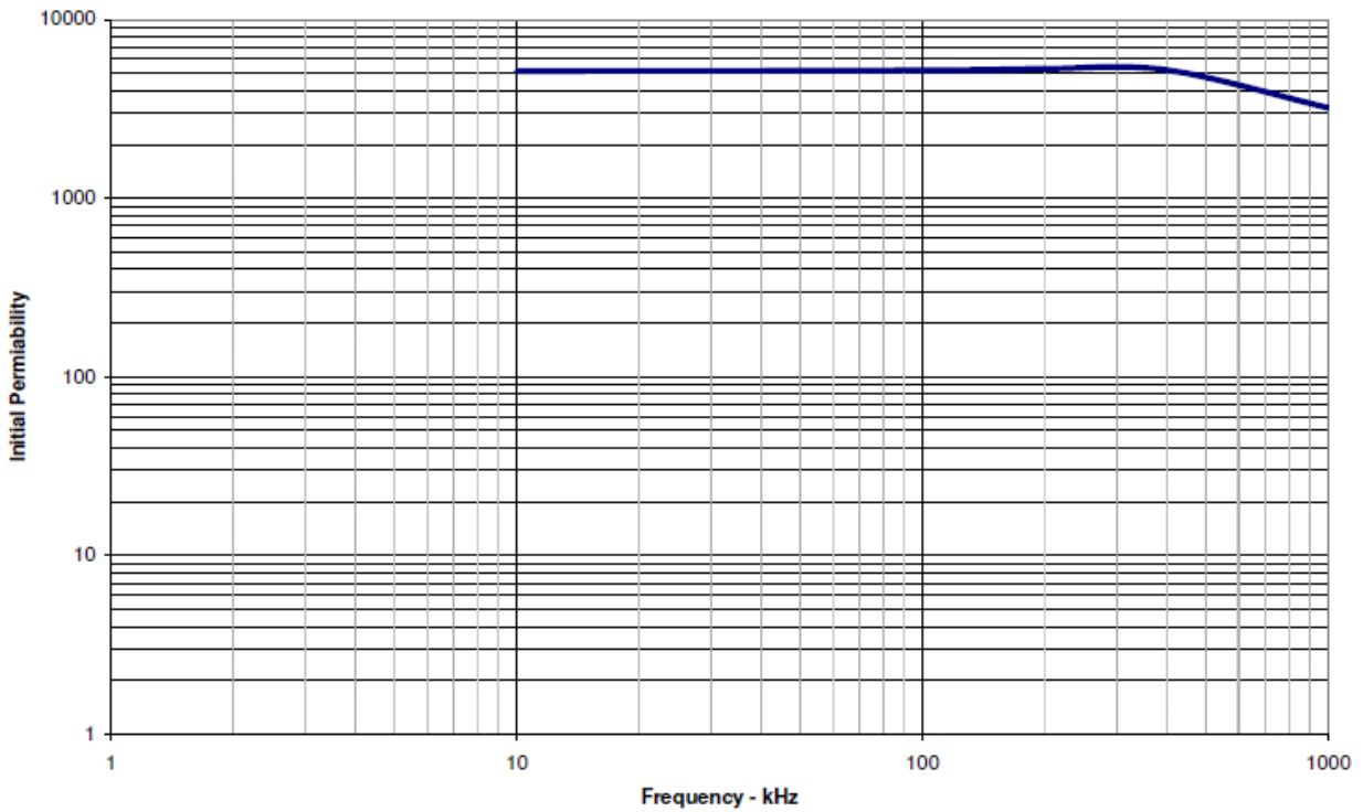
Initial Permeability versus frequency (Measured on T 2512 Toroids)
